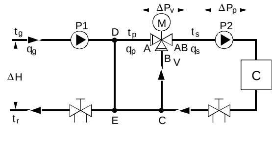
Fig. 21: Constant flow in primary/secondary circuit
