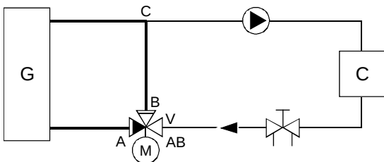
Fig. 6: Diverting three way valve
