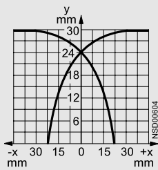
Operating distance 30 mm (normal) 3RG 40 33, 3RG40 42
