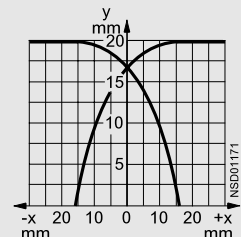
Operating distance 20 mm (extra duty) 3RG41 38
