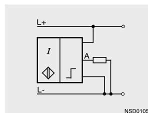
3-wire, DC, pnp, load connected between A and L-
