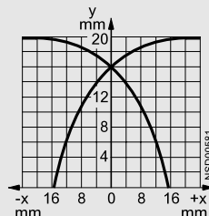
Operating distance 20 mm (extra duty) 3RG 41 34, 3RG46 38
