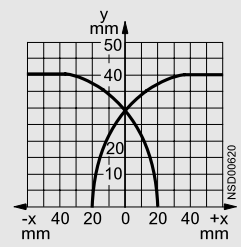
Operating distance 40 mm (extra duty) 3RG41 41
