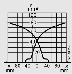
Operating distance 75 mm (U BERO) 3RG46 43
