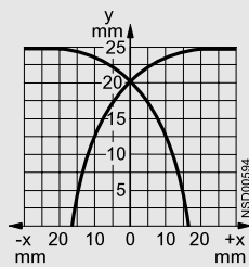
Operating distance 25 mm (normal) 3RG40 32
