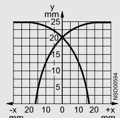
Operating distance 25 mm (extra duty) 3RG41 31, 3RG41 41
