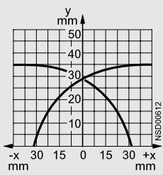
Operating distance 35 mm (U BERO) 3RG46 48
