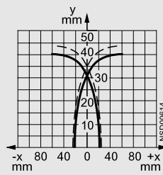
Operating distance 40 mm (extra duty) 3RG46 24
