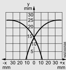
Operating distance 25 mm (U BERO) 3RG46 44, 3RG46 48
