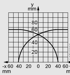
Operating distance 65 mm (extra duty) 3RG41 43
