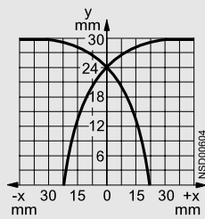
Operating distance 30 mm (extra duty) 3RG41 44
