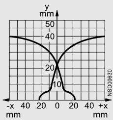
Operating distance 40 mm (U BERO) 3RG46 44
