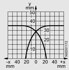
Operating distance 35 mm (extra duty) 3RG41 48
