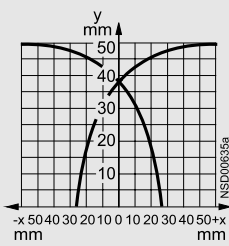
Operating distance 50 mm (extra duty) 3RG41 42
