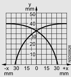
Operating distance 40 mm (normal) 3RG 40 33, 3RG40 43
