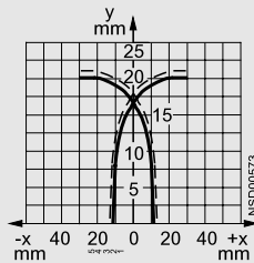
Operating distance 20 mm (extra duty) 3RG46 23
