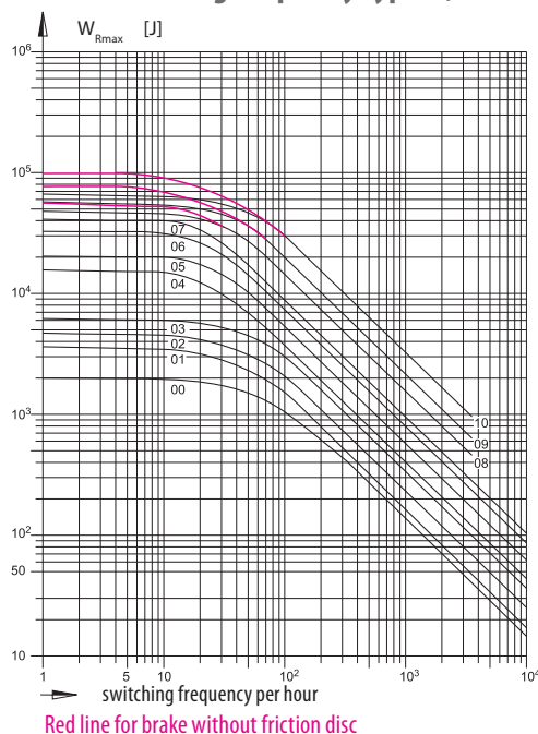
Friction switching frequency Type M, T
