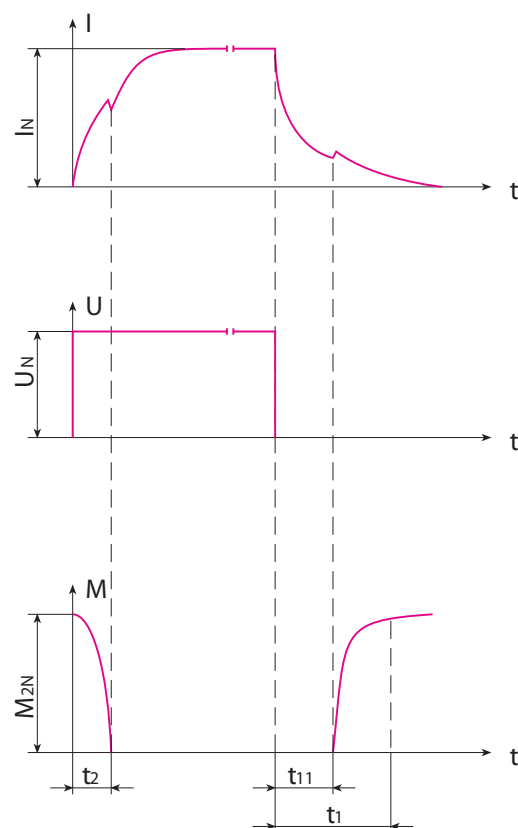
Current-time-/Voltage-time-/Torque-time-diagram
