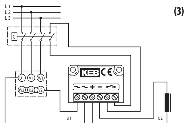
Wiring diagram
