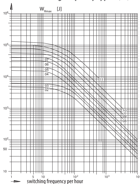
Friction switching frequency Type N, H, D
