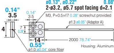
FU-54TZ Free-cut Set of 2
