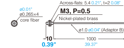
FU-79 Free-cut Set of 2
