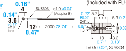
FU-53TZ Free-cut Set of 2
