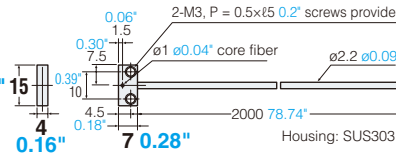
FU-54TZ Free-cut Set of 2
