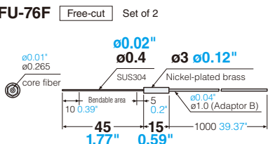
FU-76F Free-cut Set of 2
