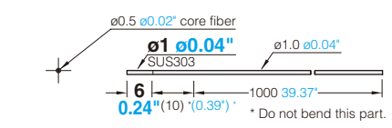
FU-58U Free-cut Set of 2
