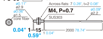
FU-88 Free-cut Set of 2
