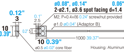
FU-51TZ Free-cut Set of 2
