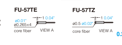
FU-57TE/57TZ Free-cut Set of 2
