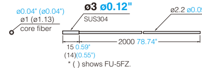
FU-5F/5FZ Free-cut Set of 2
