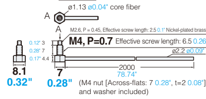
FU-77TZ Free-cut Set of 2
