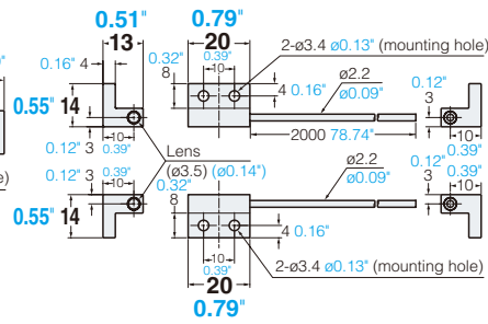
FU-L50Z Free-cut Set of 2
