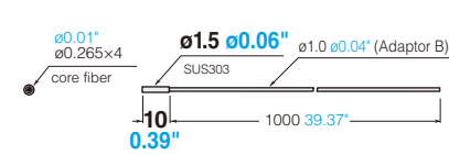
FU-59 Free-cut Set of 2
