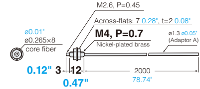
FU-78 Free-cut Set of 2
