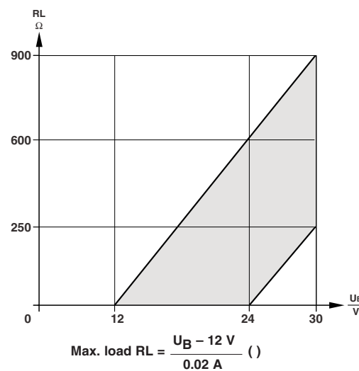
Characteristic load curve
