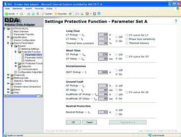
Breaker Data Adapter – device parameters
