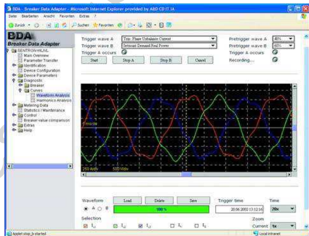
Breaker Data Adapter – diagnostics
