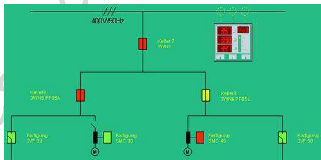
The linking of the circuit-breakers to operating and monitoring systems provides transparent power distribution
