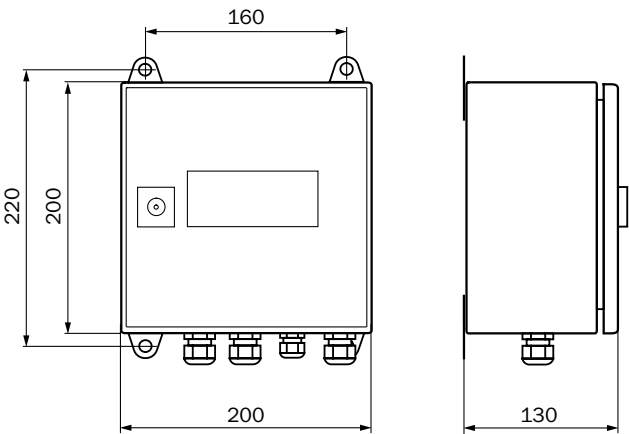
Connection unit AK1-N
