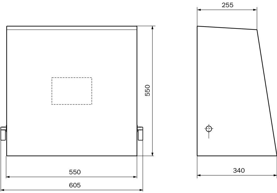
Weather hood for purge air unit SLV4/SLV5
