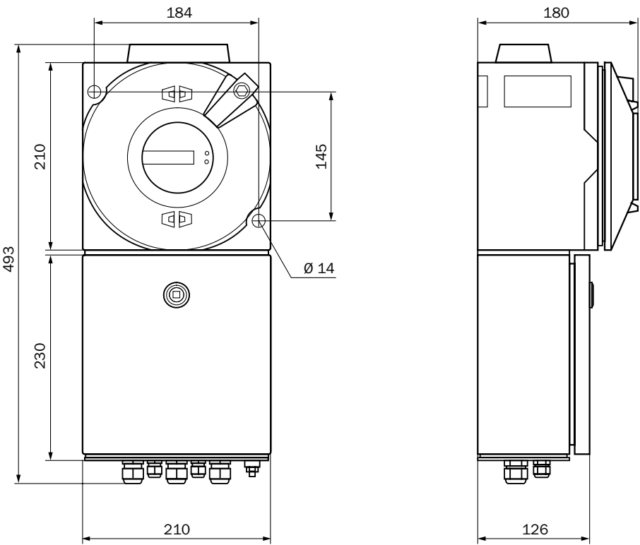
Connection unit AK1-Ex
