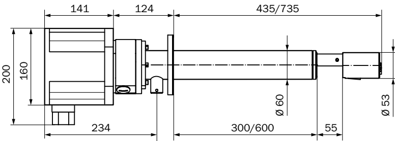
Sender/receiver unit FWSE101 Ex
