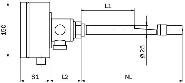
FW102 with 1" thread
