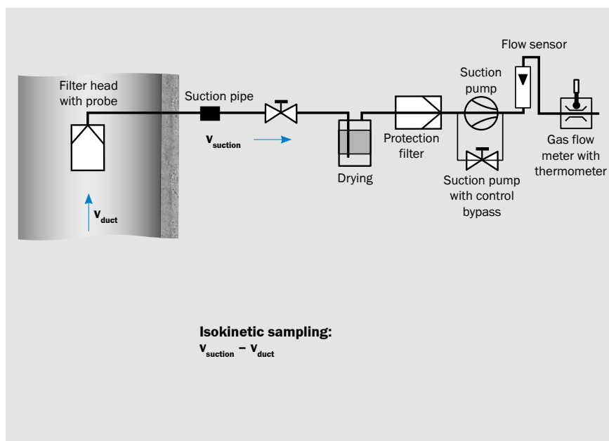
Basic setup of sampling equipment according to VDI 2066
