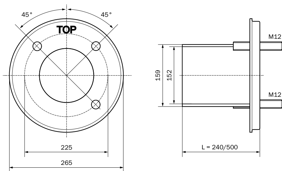
Mounting flange, D_f=152 mm
