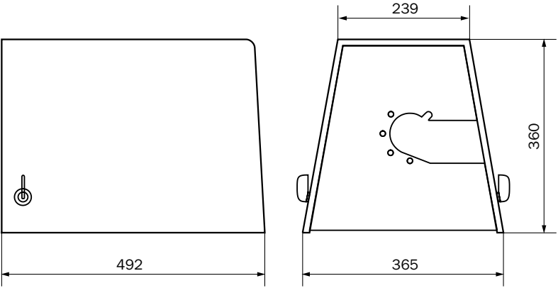
Weather hood for sender/receiver unit
