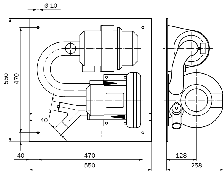
Purge air unit SLV4 2BH1300, 3-ph
